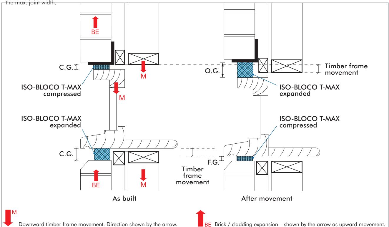
Diagram of window head and cill with masonry cladding showing before and after vertical movement. C.G. Initial Construction Gap – “before”, F.G. Final Gap – post-movement – “after”, O.G. Opened Gap – post-movement – “after”
